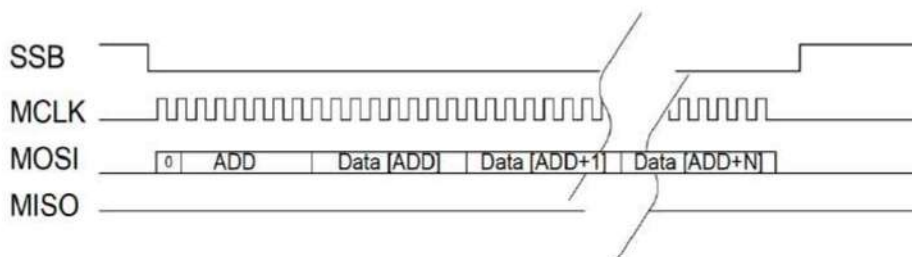
Figure 6: SPI Communication for register write access timing diagram
