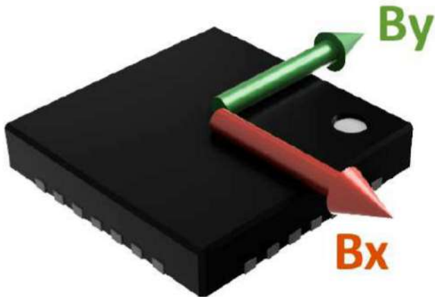
Figure 2: The two vertical Hall elements are sensitive in parallel to the chip/package surface.
